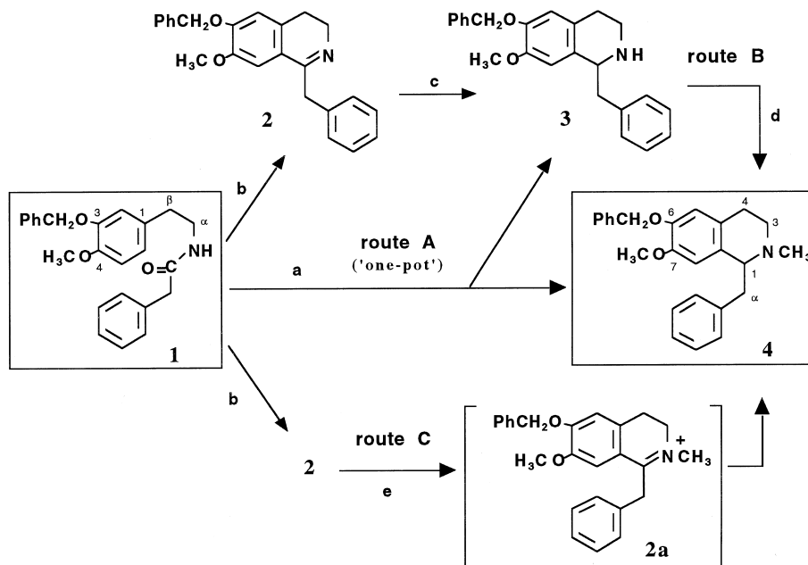
Figure 2. Syntheses of N -methyl-BTHIQ derivative 4 . Reagents and conditions: (a) \text{POCl}_3/\text{CH}_2\text{Cl}_2 , reflux, 3 h, followed by \text{NaBH}_4/\text{MeOH} , -40^\circ\text{C} , 5 h; (b) \text{POCl}_3/\text{CH}_2\text{Cl}_2 , reflux, 3 h; (c) \text{NaBH}_4/\text{MeOH} , rt, 2 h; (d) \text{POCl}_3/\text{MeOH} , rt, 30 h; (e) \text{POCl}_3/\text{MeOH} , reflux, 9 h, followed by \text{NaBH}_4 , rt, 3 h.
